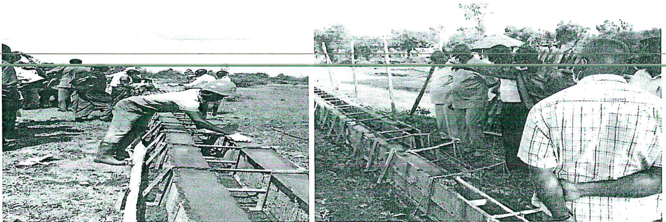
Construction of Minor canals in Kimira Scheme (BL 7) and The Monitoring team from SDRNCD inspecting the same
