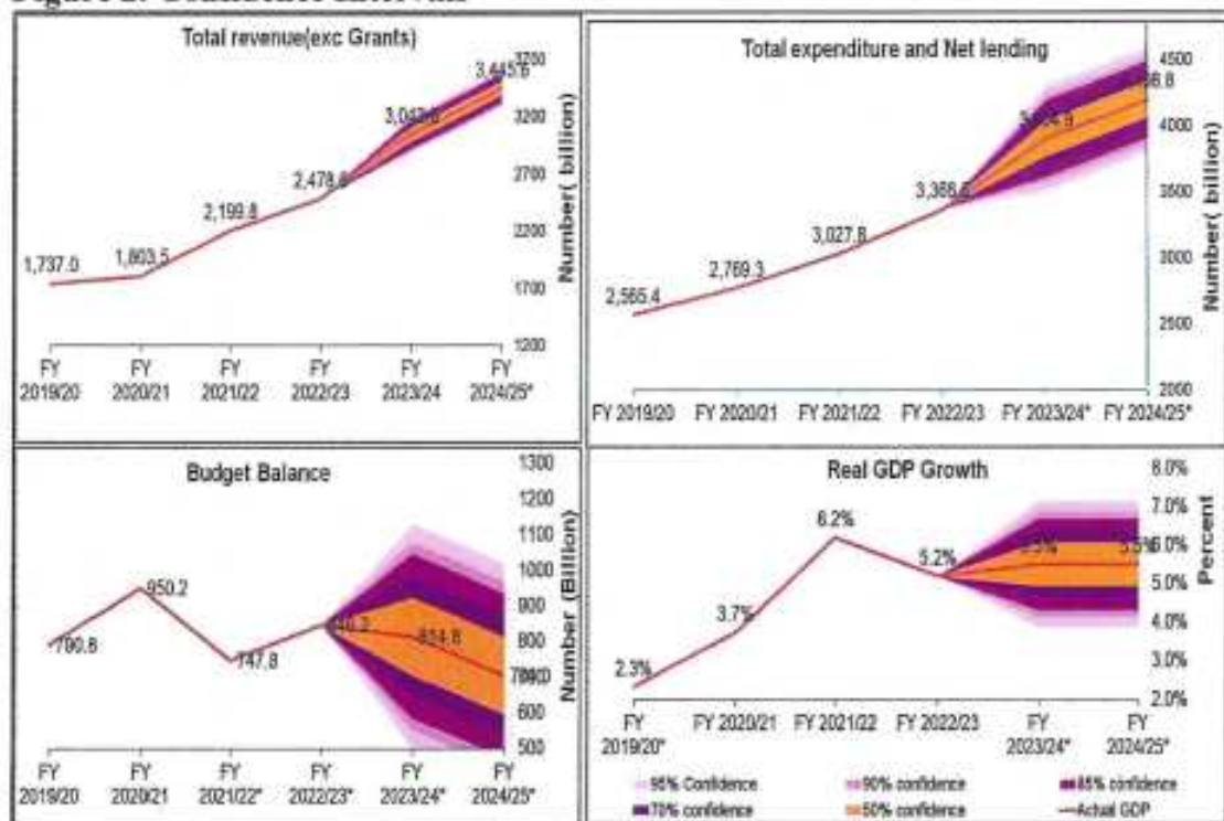
Figure 2: Confidence Intervals
